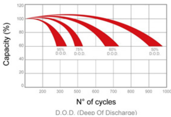
Charge Cycles (25°C)
