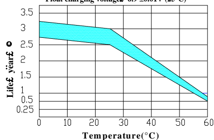
Temperature effect on float life Float charging voltage ± 6.9 ± 0.01V (25°C)
